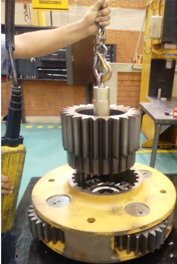
INSTALL SUN GEAR
